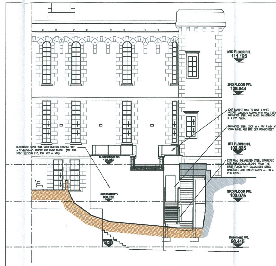
Block H: Stores Building - North Facing Elevation 1:75
