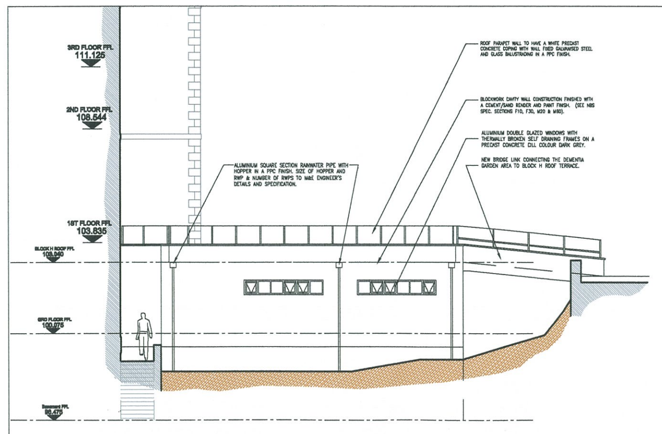
Block H: Stores Building - East Facing Elevation 1:75
