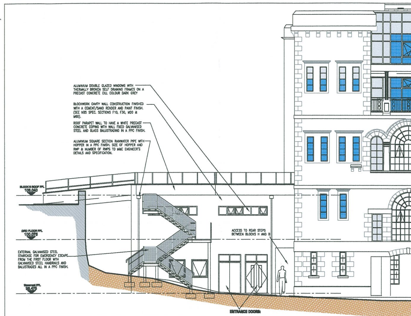
Block H: Stores Building - West Facing Elevation 1:75
